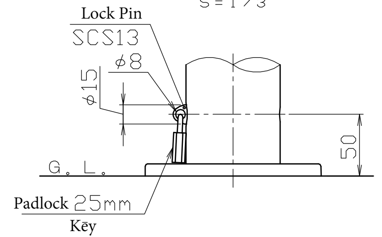
Details of Base S = 1 / 3
