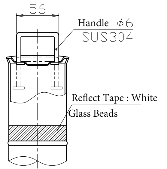
Details of the Handle on Top Part S = 1 / 3
